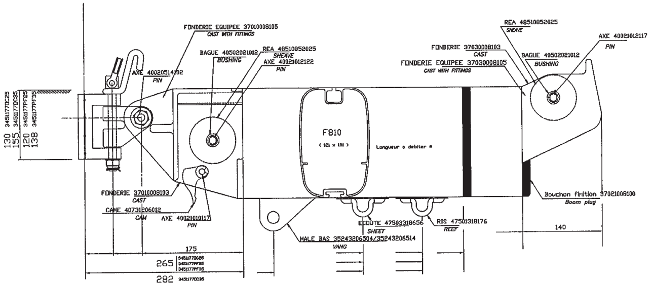
VIT DE MULET COMPLET 3451177DC25 / 3451177DC35 3451177PF25 / 3451177PF35 COMPLETE GOOSENECK
