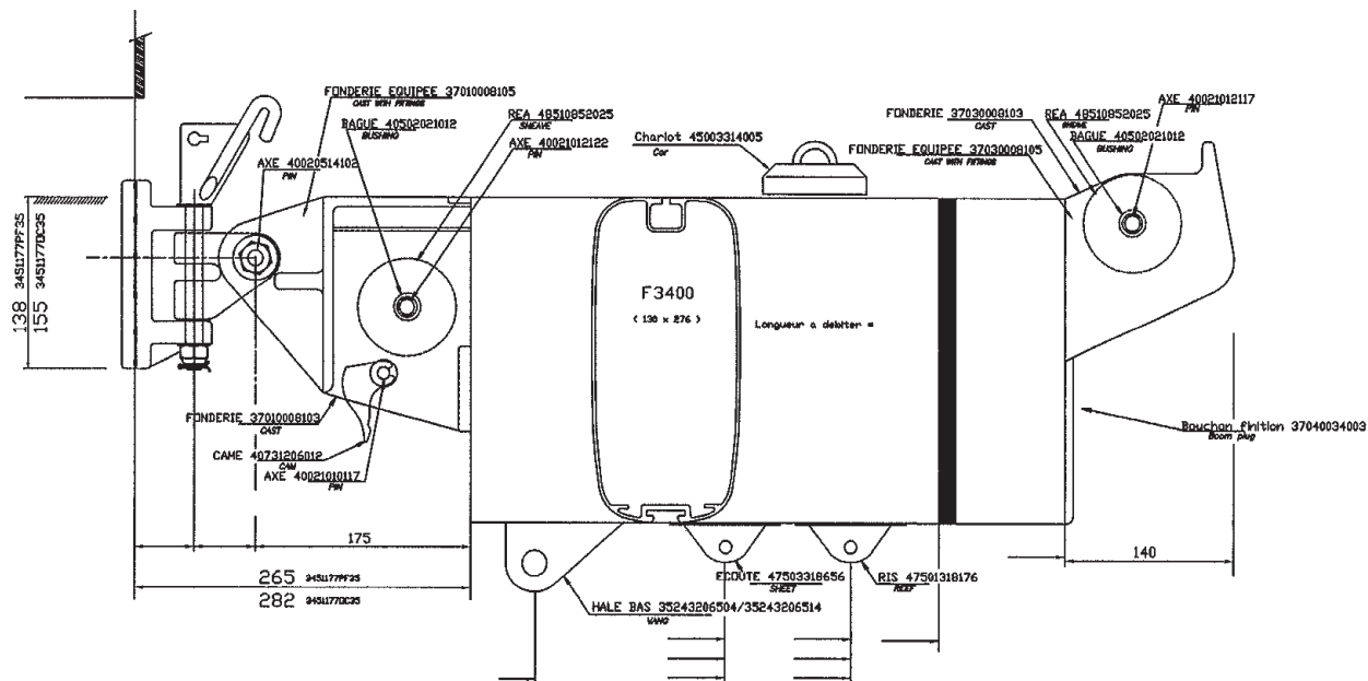
VIT DE MULET COMPLET 3451177PF35 / 3451177DC35 COMPLETE GOOSENECK
